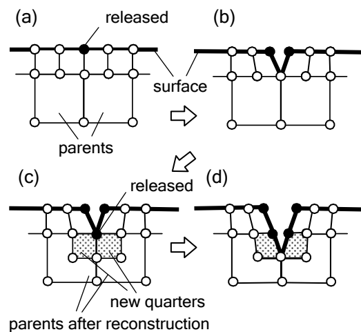
Figure 7. Generation of quarter elements in the reconstruction procedure.
