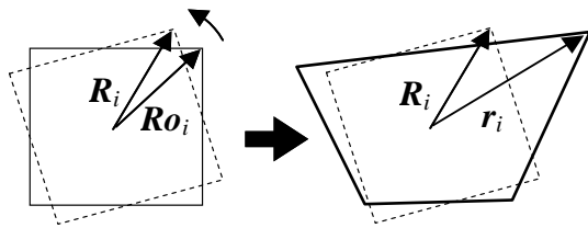
Figure 1. Vertex displacements in a volumetric elasticity element. Solid lines show the original reference shape, broken lines show the rotated reference shape, and bold lines show the deformed shape.
