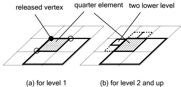
Figure 6. Conditions for generating quarter elements in the reconstruction procedure.
