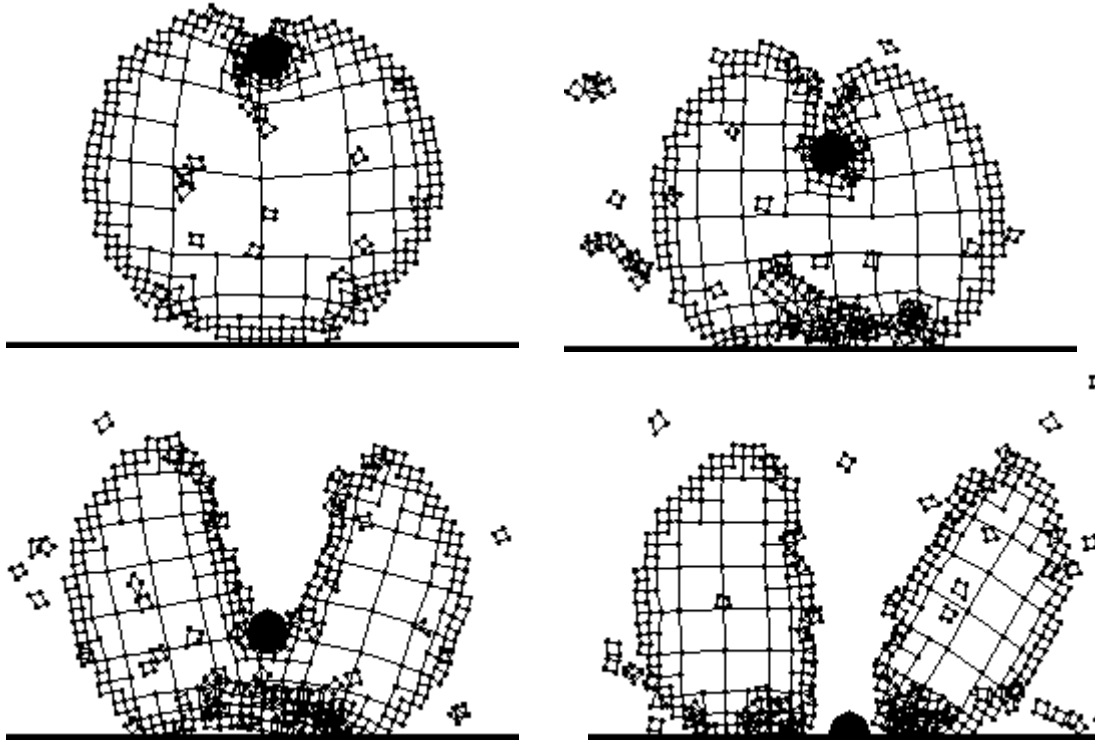
Figure 8. Reconstruction process according to cutting operation.
