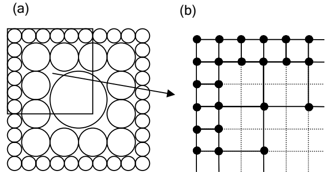
Figure 2. Image illustrations of a gradational element resolution model. (b) is a magnified illustration of a corner of a cubic object (a).
